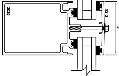
2 2 PARTER DETAIL SCALE: FULL
