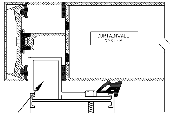
MAJOR INDUSTRIES GUARDIAN 275 ® TRANSLUCENT WALL PANEL SYSTEM
