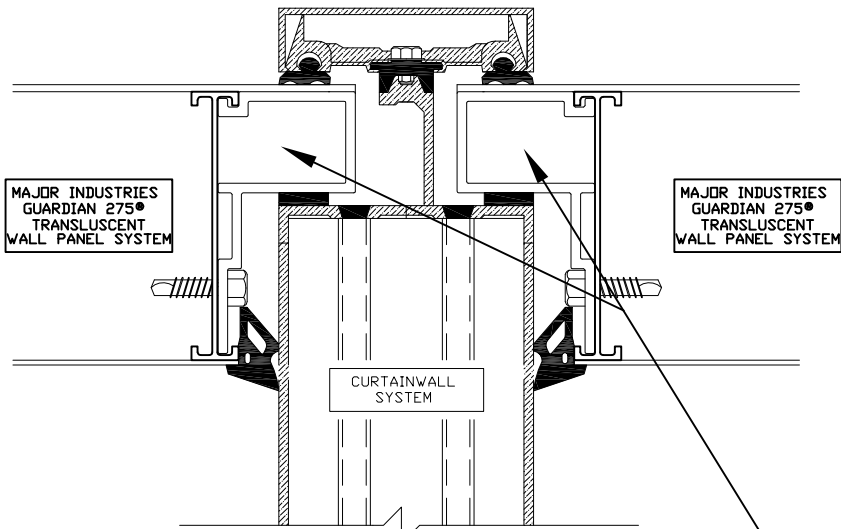
MULLION / PURLIN DETAIL
