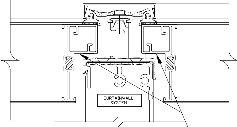
MULLION / PURLIN DETAIL
