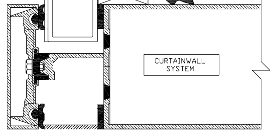
HEAD & SILL DETAIL
