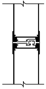
MATING BAR DETAIL SCALE: NTS
