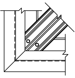
HIP CONNECTION SCALE: NTS
