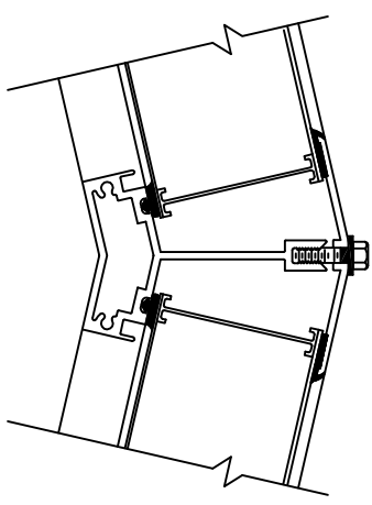
1 HIP DETAIL SCALE: NTS
