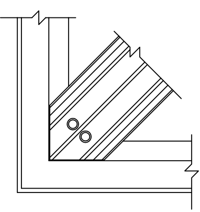
2 HIP CONNECTION SCALE: NTS
