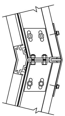
4 COMPRESSION CONNECTION SCALE: NTS
