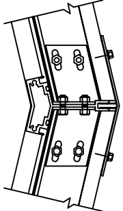
COMPRESSION CONNECTION SCALE: NTS
