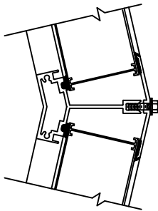
2. HIP DETAIL SCALE: NTS
