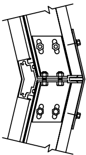
5. COMPRESSION CONNECTION SCALE: NTS
