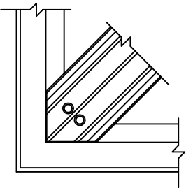
4. HIP CONNECTION SCALE: NTS
