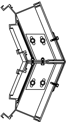
11-11 COMPRESSION CONNECTION SCALE: NTS
