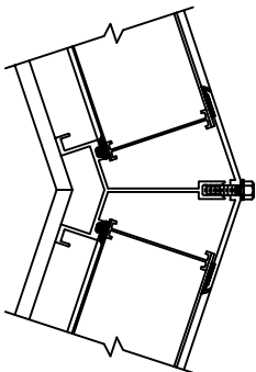
HIP DETAIL SCALE: NTS
