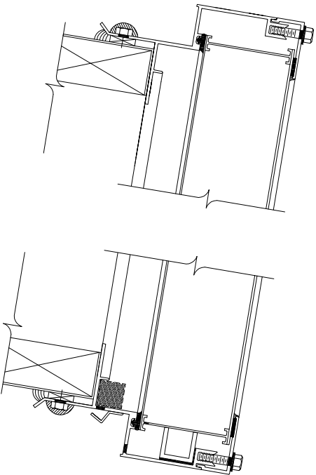
2 1 - - SILL DETAIL
